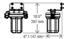
Sea Strainer
