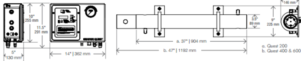
Right Side View
