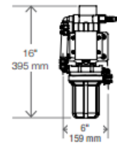
Fresh Water Flush (optional)
