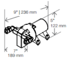
Booster Pump Assembly (optional)
