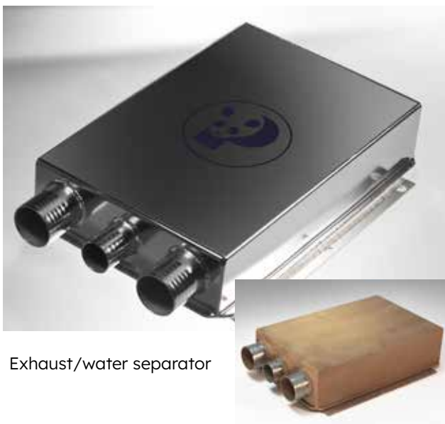
Exhaust/water separator with noise reduction coating
