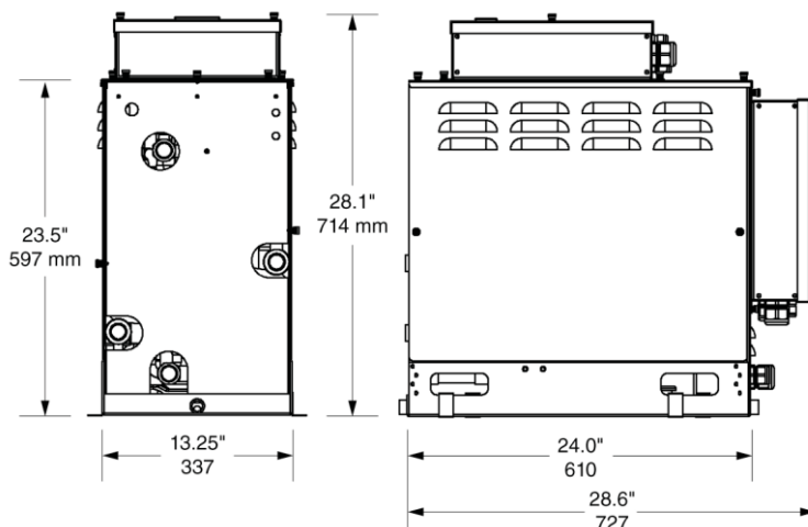
VARC 72 Electrical Box
