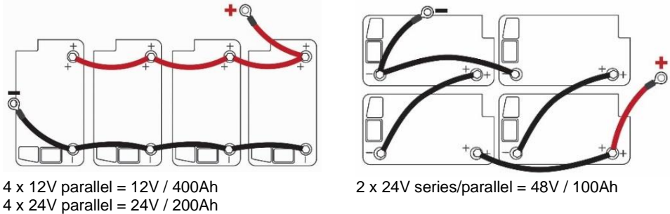
Figure 10: Simplified diagram for battery bank DC connections
